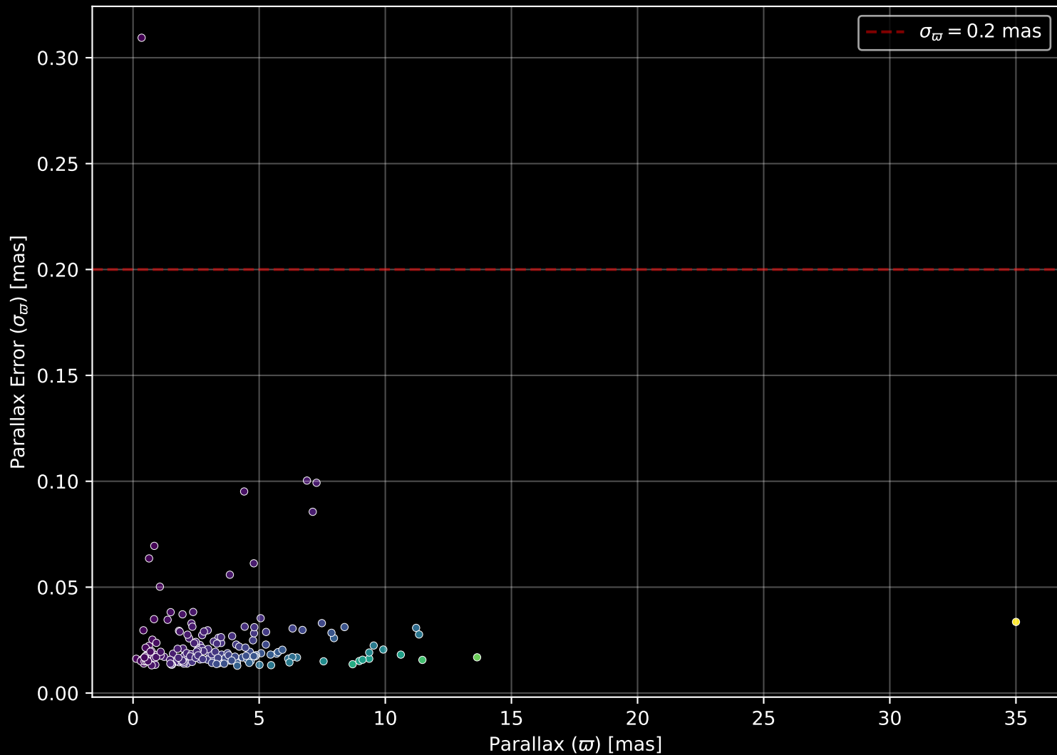
APOGEE DR17 Field: [187+48_MGA] Parallax Quality (n= 176)
