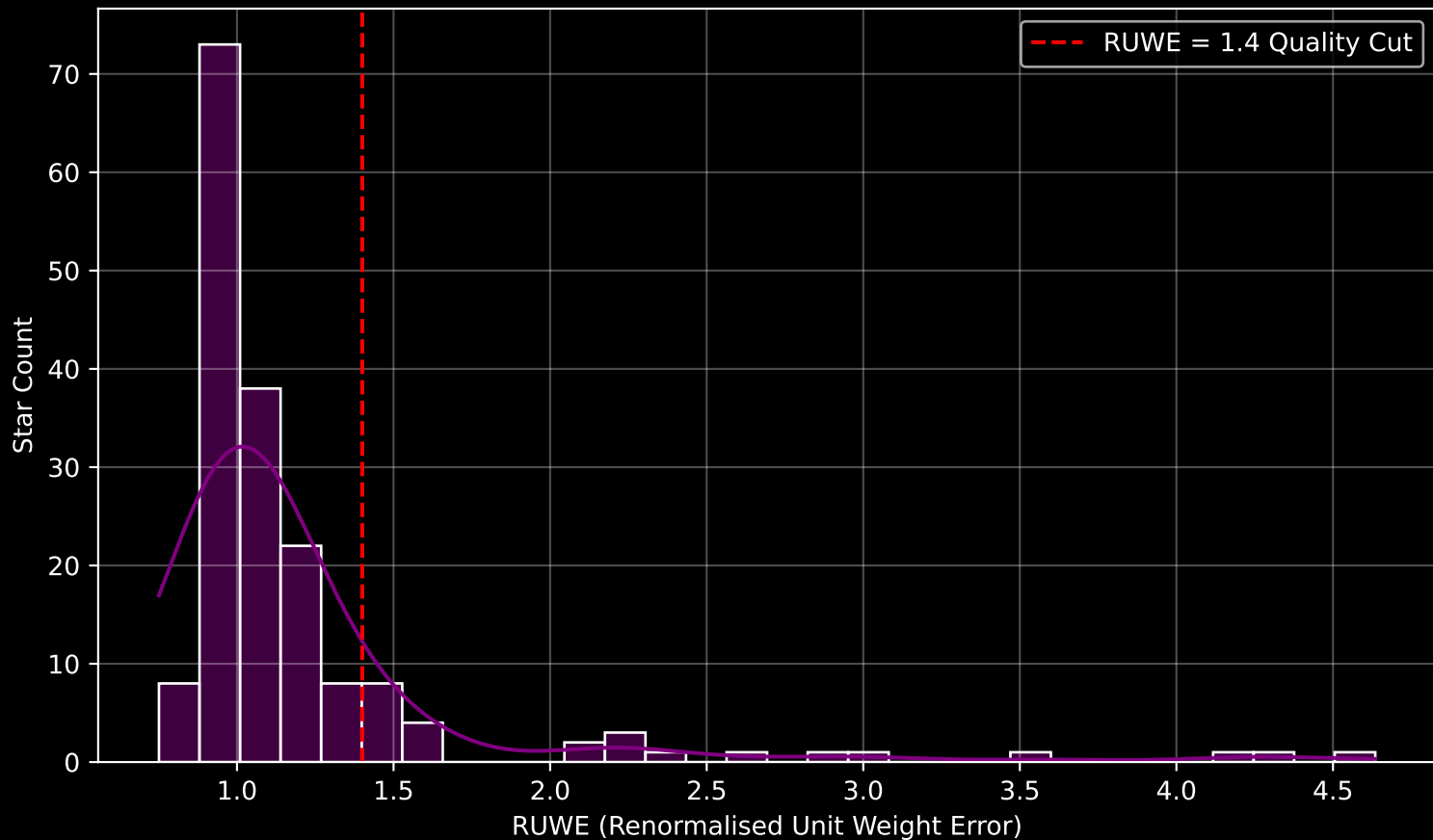
GAPOGEE DR17 Field [187+48_MGA] RUWE Distribution (n= 174)
