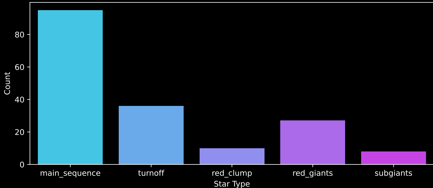
APOGEE DR17 Field: [187+48_MGA] Count plot of Star Type
