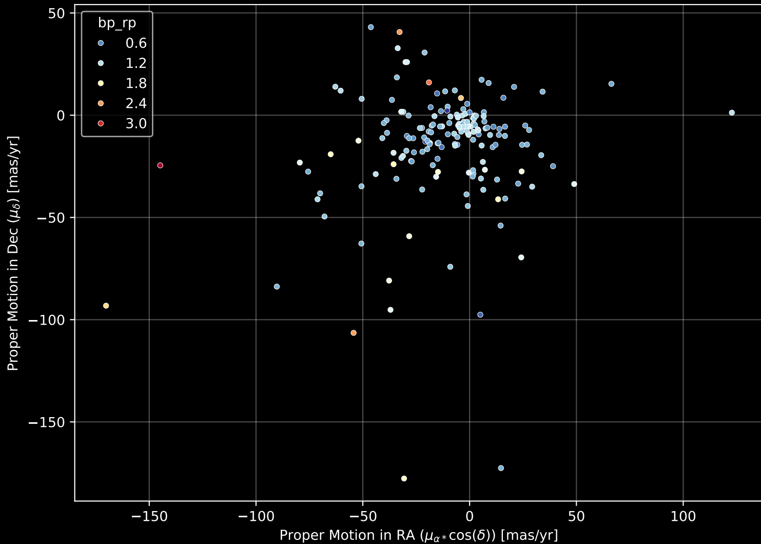
APOGEE DR17 Field: [187+48_MGA] Proper Motion Diagram (n= 176)
