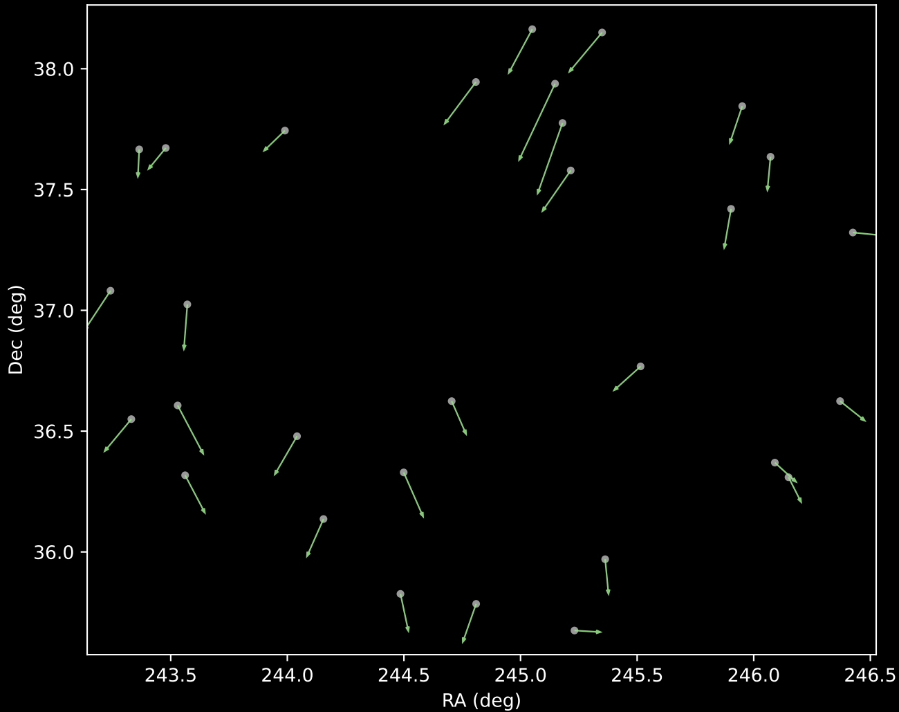
APOGEE DR17 Cluster 5 Proper Motion Vectors (n=30)
