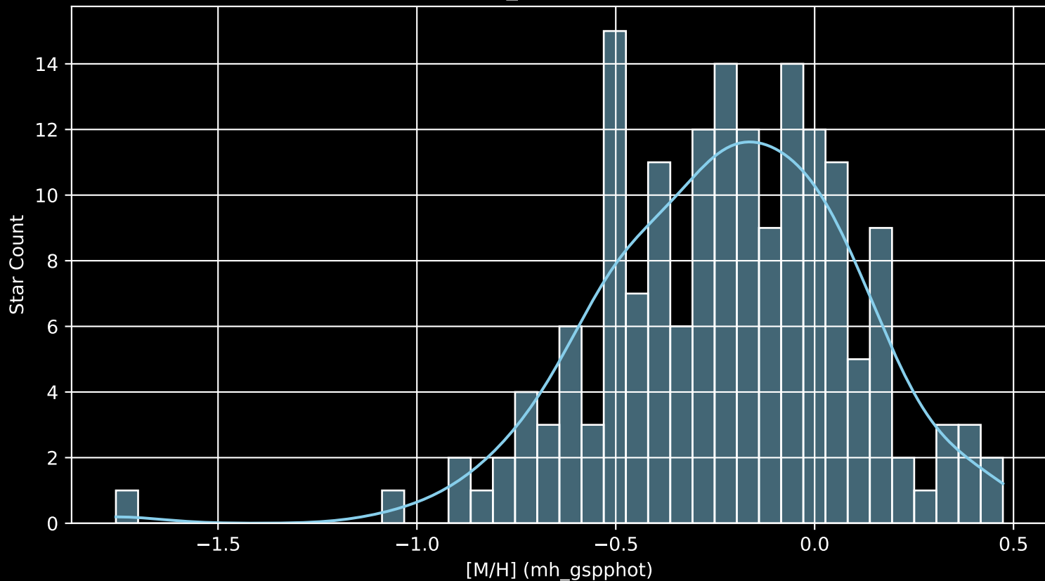
APOGEE DR17 Field: [187+48_MGA [M/H] (mh_gspphot) (n= 171)
